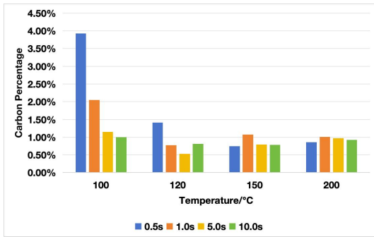
Fig.3 Percentage of residual carbon in the Al 2 O 3 film with different temperature and H 2 O vapor dose
