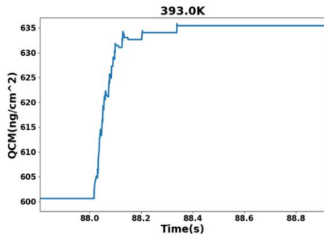
Fig.1 Time evolution of TMA adsorption by Kinetic Monte Carlo simulation
