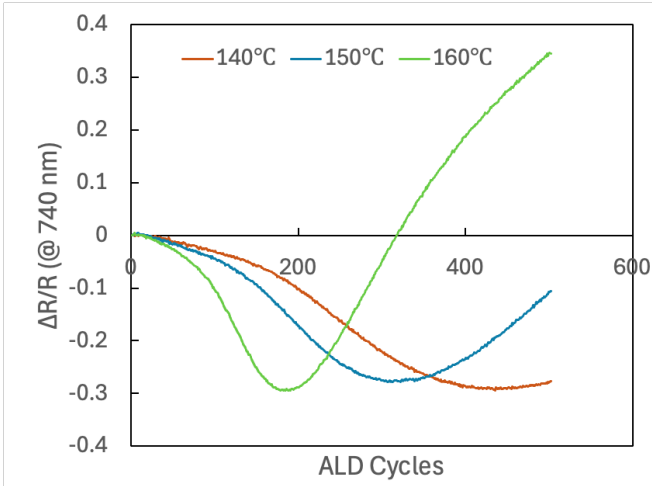
Figure 1. Reflectance changes at a wavelength of 740 nm during 500-cycle Cobalt ALD
