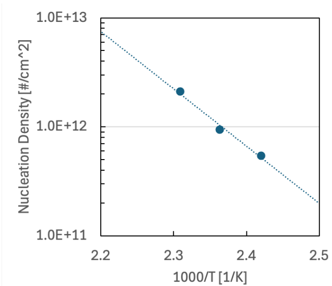
Figure 3. Arrhenius plot of the initial nucleation density
