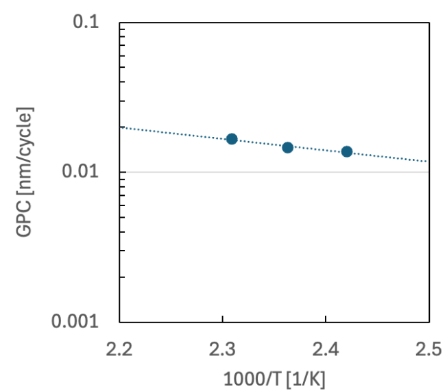
Figure 2. Arrhenius plot of the growth per cycle
