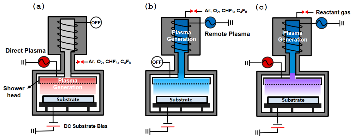
Fig 1. Schematics of plasma power supplies used in this study. Equipment used for (a) DPALE, (b) RPALE, and (c) CPALE
