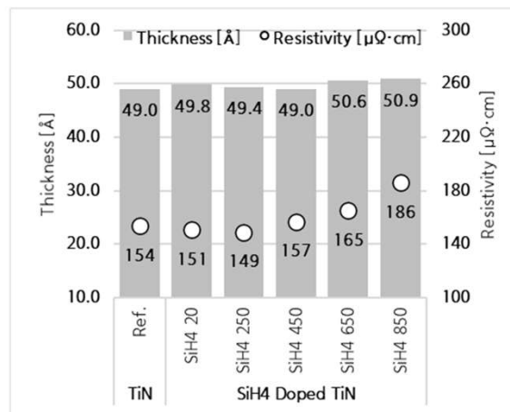
Figure 1. Resistivity of TiN films vs SiH 4 flow rate (20-850 sccm) at 550°C
