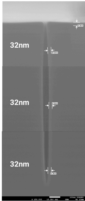
Step coverage of Nb 3 at 350°C : 100% (A/R = 1:30)
