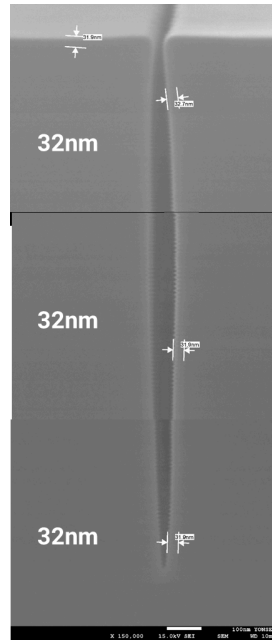
Step coverage of Nb 3 at 375°C : 100% (A/R = 1:30)
