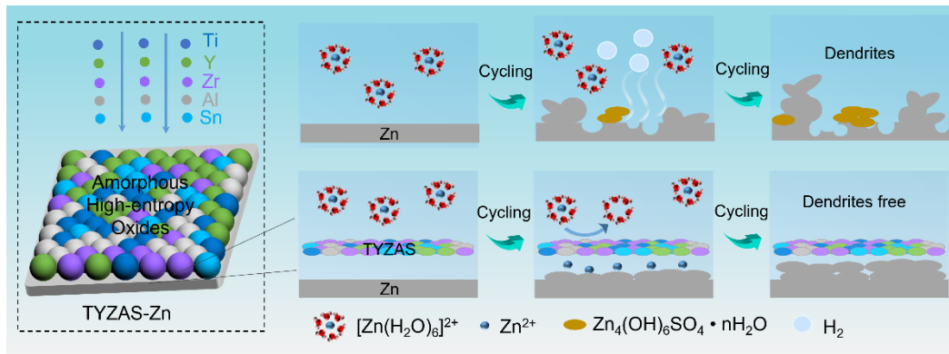
Fig. 1. Schematic of electrochemical galvanization on bare zinc and TiYZrAlSnO x electrodes.
