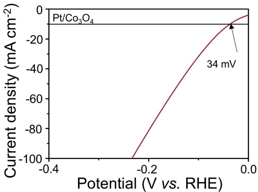
Figure 1. Polarization curve obtained by LSV testing of the Pt/Co 3 O 4 sample with Pt source pulse time of 300s.
