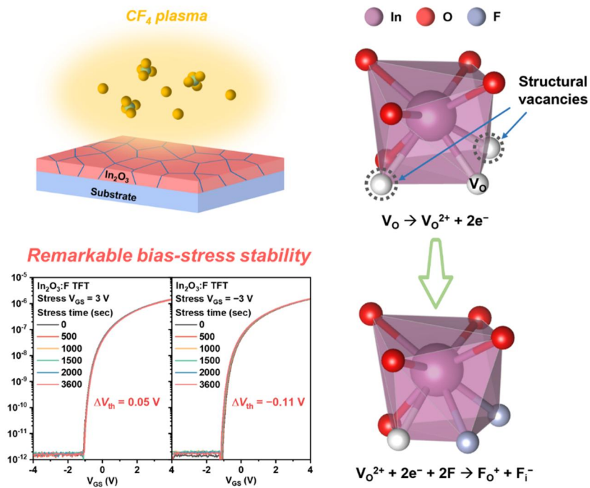
Figure 1. Schematic illustration of the plasma fluorination strategy to achieve both high performance and high stability for In 2 O 3 :F TFTs.
