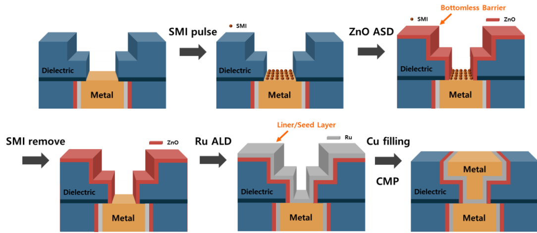
Figure 1. Schematics of the process for forming the Ru/ZnO bottomless barrier bilayer in a Cu via
