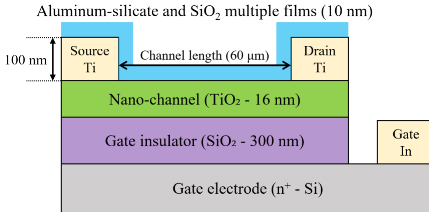
Fig.1 Schematic of TiO 2 -TFT with aluminum-silicate and SiO 2 multiple films.
