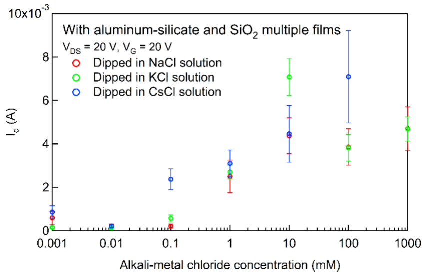
Fig.2 Correlation between alkali-metal chloride concentration and drain current. TiO 2 -TFT with aluminum-silicate and SiO 2 multiple films.
