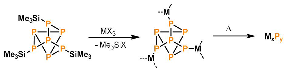
Fig. 1. Representative reaction of P 7 (SiMe 3 ) 3 with a metal halide to generate a metal phosphide.
