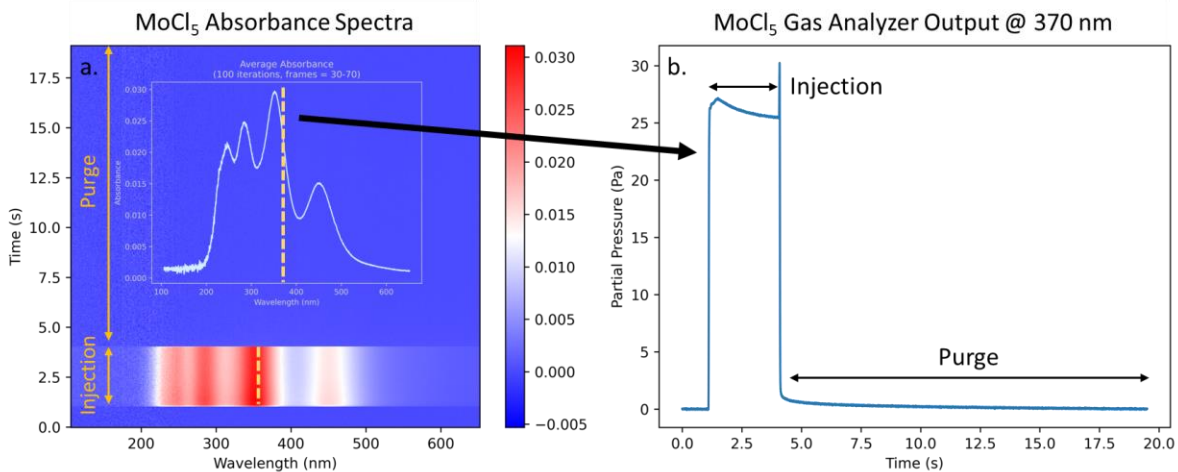
Figure shows (a) time-resolved absorbance spectra obtained during a 3.0 s injection of MoCl 5 at a vessel temperature of 110 °C and using 100 sccm of Ar carrier gas. The corresponding data from the MoCl 5 gas analyzer is shown in (b). Both plots represent an average of 100 injections.
