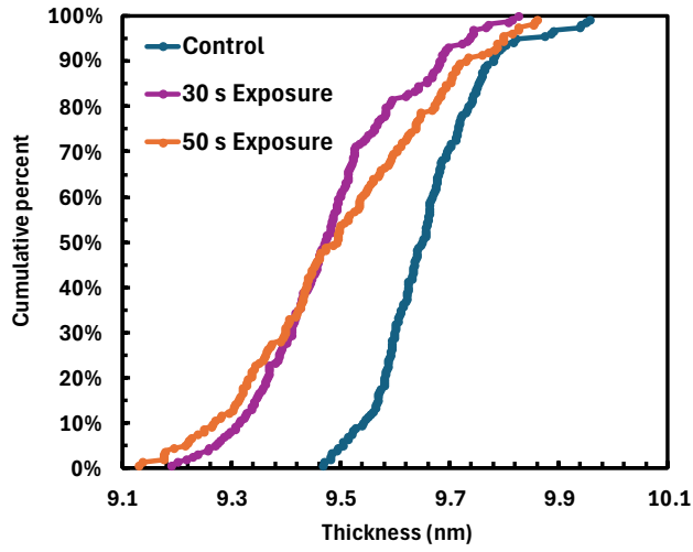
Fig. 1. Cumulative percentage of sites measured vs. \text{Al}_2\text{O}_3 film thickness across 150 mm Si wafer, captured using a mapping ellipsometer, for 100 cycle films deposited without (control) and with 30 sec and 50 sec of microwave exposure performed during the TMA purge of each cycle.
