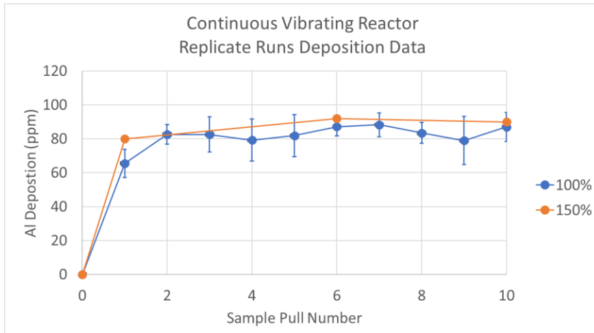
Figure 2. Measured Al loading of 4 ALD Al 2 O 3 cycles graphite for 3 replicate coating runs (10 pulls per run) with TMA flow rates at 100% surface titration and 1 run at 150% surface titration.
