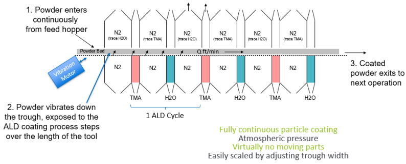
Figure 1. Schematic and photo of the spatial CVR ALD system
