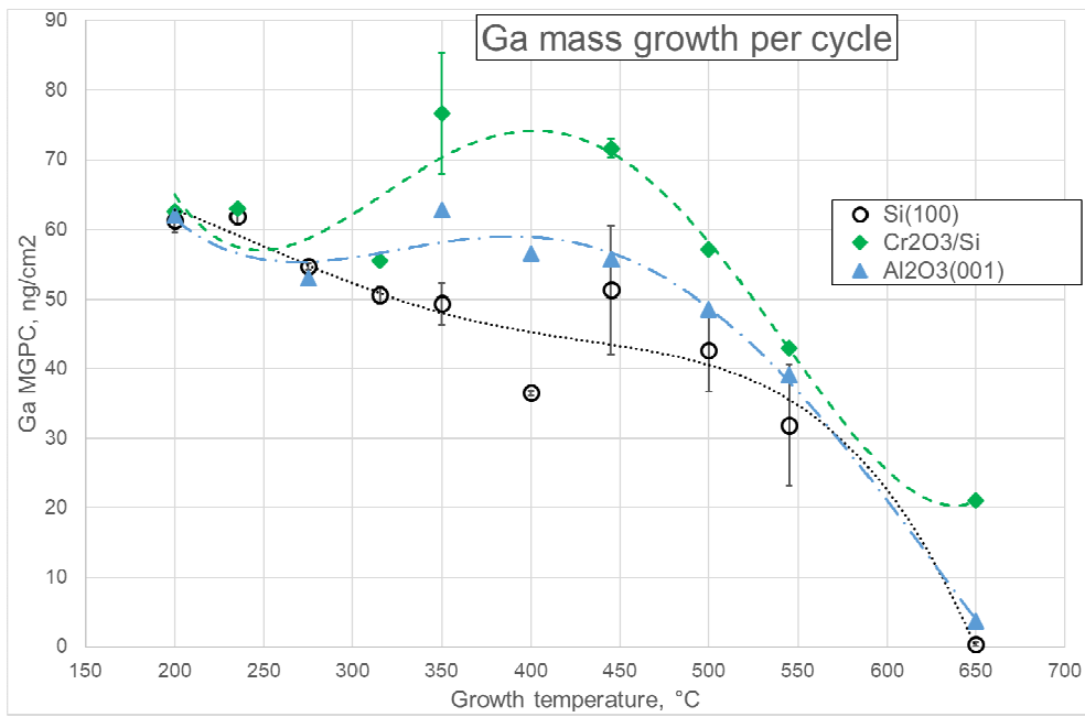
Figure 1. Dependence of growth rate on the deposition temperature. Rise of the mass growth per cycle values at around 300 °C for the films grown on \alpha -Cr 2 O 3 seed layers and on \alpha -Al 2 O 3 substrates as well as at 450 °C for the films grown on Si is related to the crystallization of the films.
