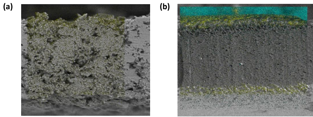
Figure 1. Cross-section SEM elemental mapping, yellow for zirconium and blue for aluminum coming from the sample holder (a) ALD deposition of zirconium dioxide on the sample with 24 aspect ratio, (b) ALD deposition of zirconium dioxide on the sample with 1000 aspect ratio
