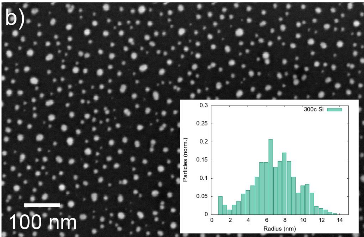
Figure: Example of ALD Au nanoparticle growth on silicon with native silicon oxide layer. Scanning electron micrographs of samples with (a) 100 and (b) 300 ALD Au cycles. The insets show the corresponding normalised particle size distributions.
