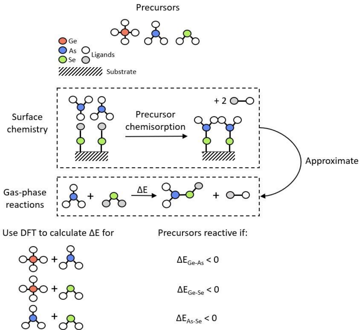
Figure 1: Schematic overview of the work is shown in which Density Functional Theory is abbreviated as DFT.
