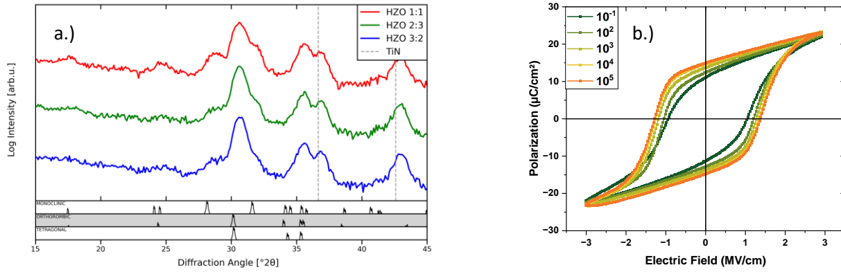
Fig 1: a.) XRD patterns of HZO samples with varying Hf:Zr ratios. b.) The Polarization-Electric field (P-E) hysteresis for the HZO 3:2, deposited at 350°C, cycled from pristine up to 10 5 cycles.
