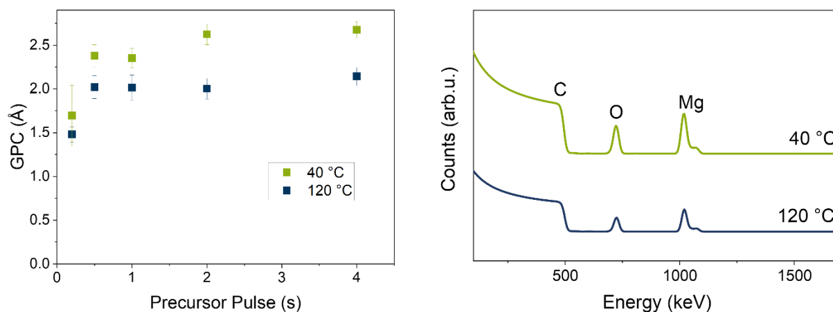
Figure 1. Saturation of the precursor pulse using [\text{Mg}(\text{DMP})_2] and \text{H}_2\text{O} on Si substrates (left) and RBS spectra of the resulting thin films on glassy carbon (right) at 40 °C (green) and 120 °C (blue).
