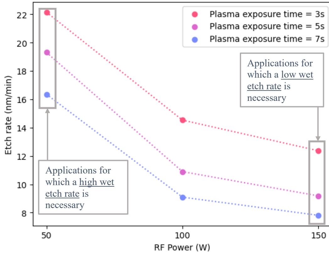
Figure 1: Dependence of RF power and plasma exposure time on wet etch rate of SiO 2
