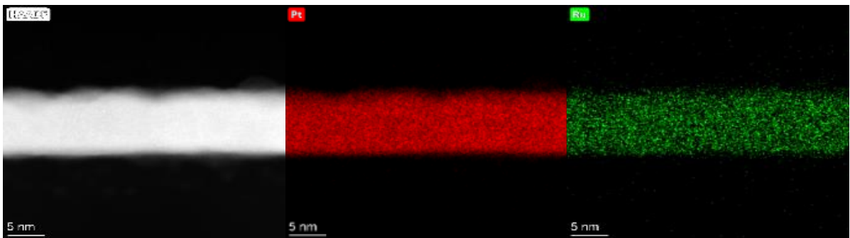
Figure 2. XTEM images of PtRu alloy thin films prepared by ALM. STEM-EDS mapping results clearly shows the formation of atomic-scale homogeneous alloy film.
