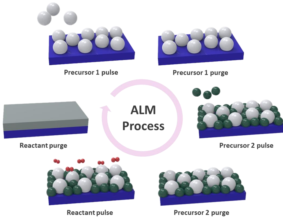
Figure 1. Schematics of ALM process steps
