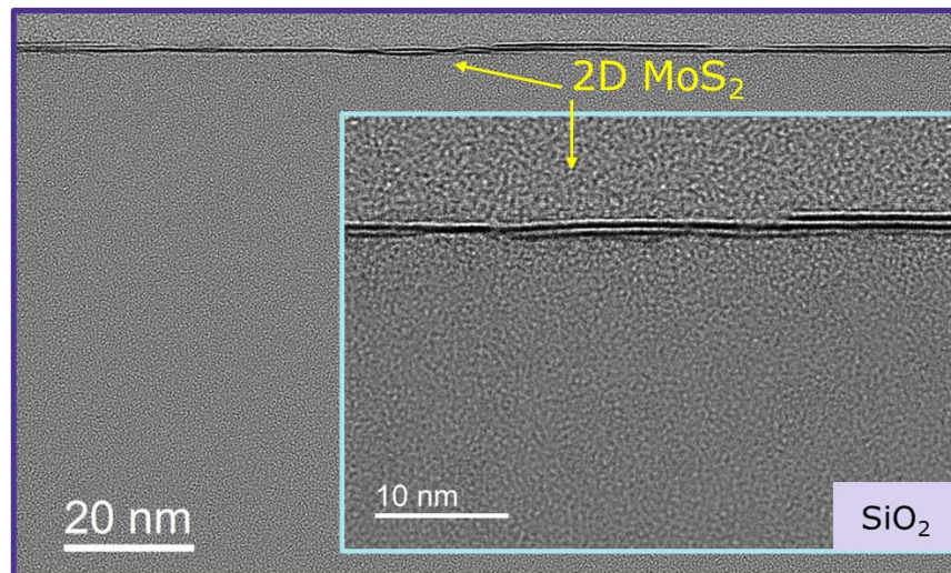
Fig. 1. Cross-section TEM image of 2D \text{MoS}_2 deposited on 3\text{k}\text{\AA} \text{SiO}_2/\text{Si} substrate by \text{MoCl}_5 -based thermal ALD.
