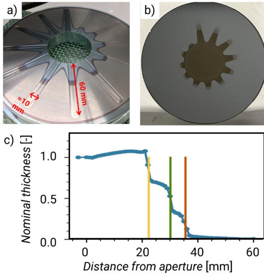
Figure 1: a) Bottom side of the HAR disk. b) A staircase pattern on a 200 mm Si wafer c) an Ellipsometer line scan of a tunnel from b). Vertical lines signify PD50s from different pulse times.
