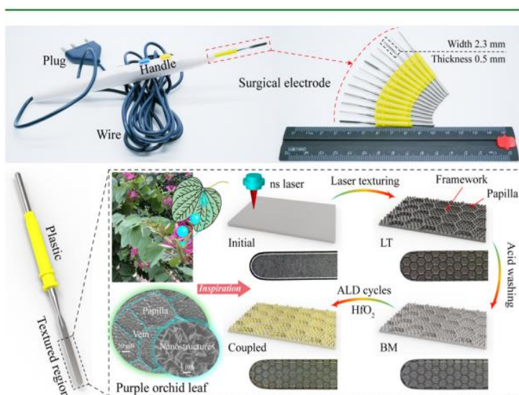
Figure 2. The fabrication process of the bionic microstructure in coupled electrode.
