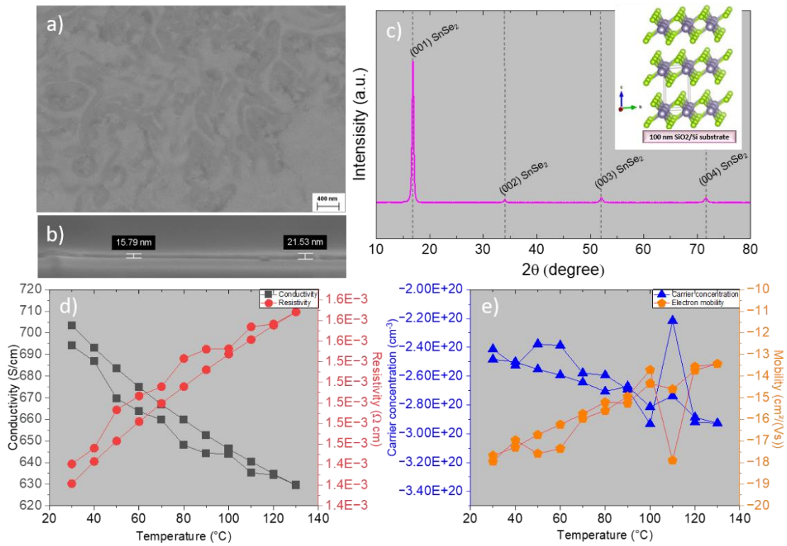
Figure 1. a) Top and b) cross view SEM images of a 20 nm SnSe 2 thin film. c) XRD diffraction pattern after annealing. Plot d) shows the electrical conductivity (black squares) and resistivity (red dots) and e) carrier concentration (blue triangles) and electron mobility (orange pentagon) with increasing temperature.
