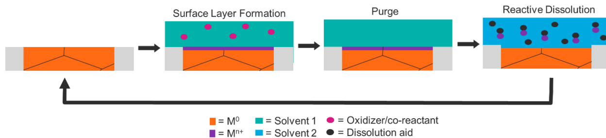
Figure 1. A diagram of the Ru wet ALE process. A surface layer is formed in the first etching solution through the reaction with oxidizers and co-reactants. The surface layer is selectively removed in a second solution through reactive dissolution.
