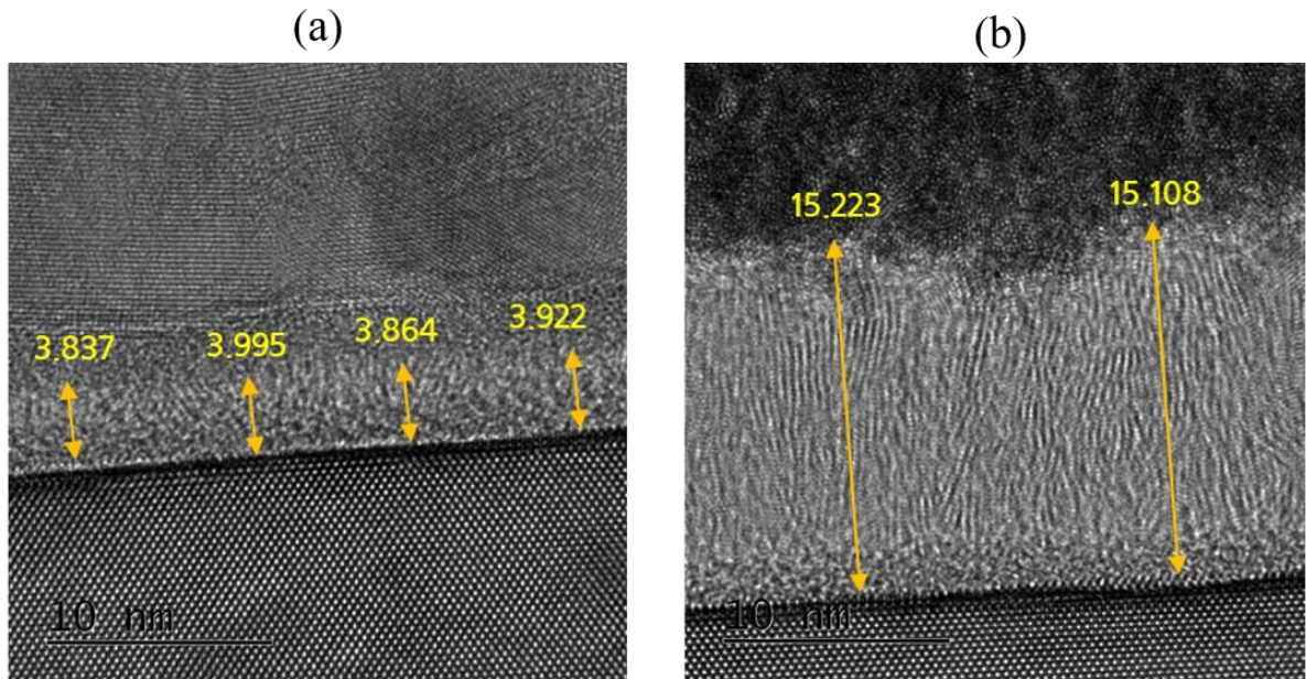
Figure 2. TEM image of (a) amorphous and (b) nano-crystalline BN
