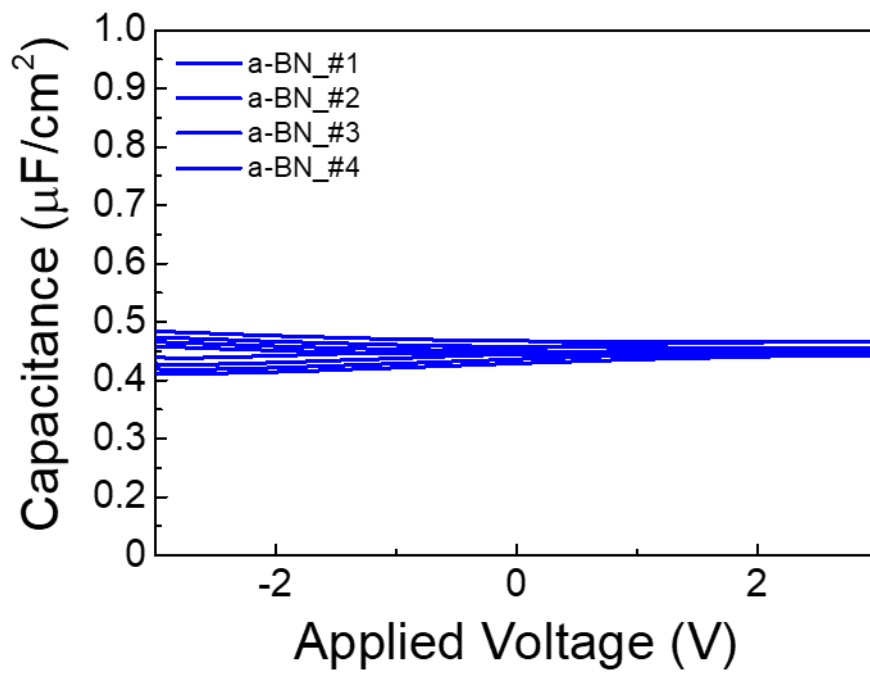
Figure 3. C-V characteristics of synthesized a-BN
