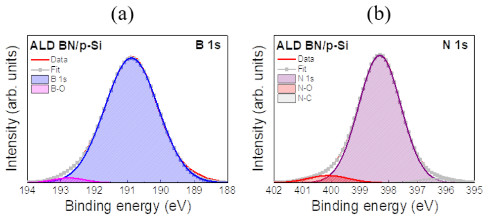
Figure 1. XPS spectra of synthesized a-BN, (a) B 1s, (b) N 1s
