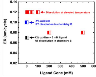
Fig.2: Mo ER as a function of ligand concentration at different dissolution temperature
