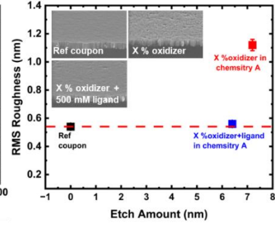
Fig.3: RMS roughness of as deposited and post-etch Mo coupon. Inset shows the SEM images of as deposited and post-etch Mo coupon under different conditions.
