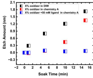
Fig.1: Mo surface oxidation as a function of soak time in different oxidizing solutions
