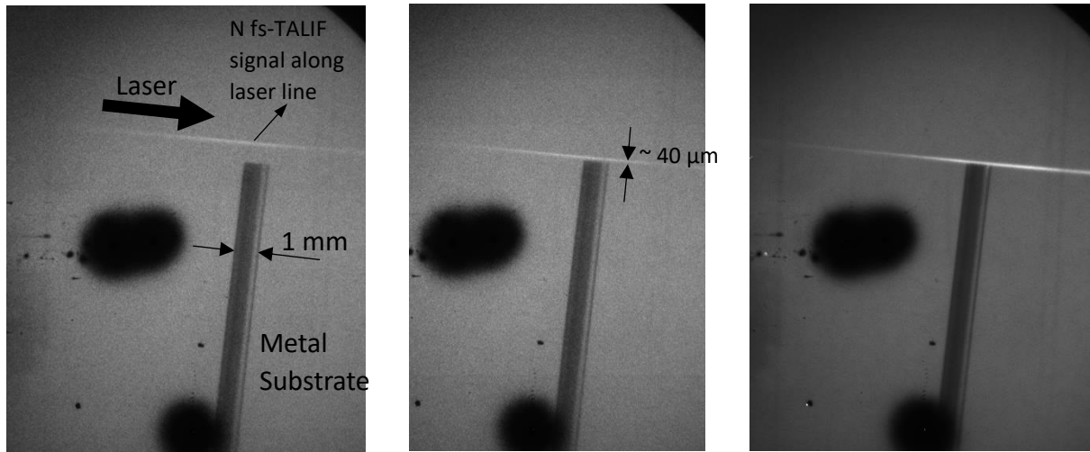
Figure 1: Sample images showing N atom TALIF signal along the laser line. The laser was aligned for grazing over the metal substrate tip. Pressure of 5 mTorr, air plasma at room temperature.
