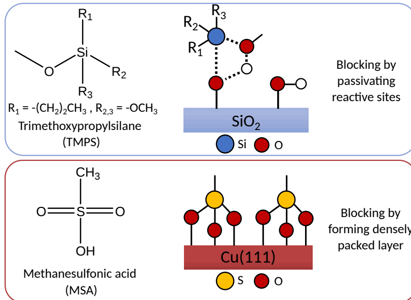
Figure 1.: Lewis structures and schematic blocking mechanism of TMPS and MSA.
