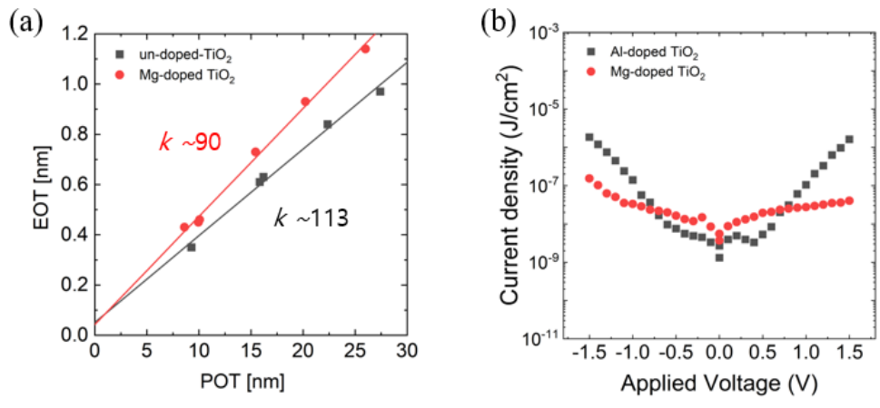
Figure 1. (a) The EOT-POT graph of the Pt/RuO 2 (MTO, TiO 2 )/Ru structure capacitor. (b) J–V curves of 20-nm-thick MTO and ATO films.
