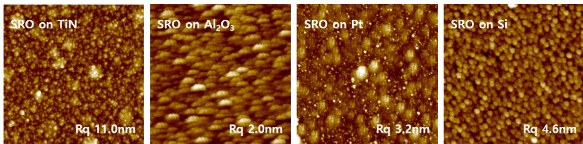
Figure 1. AFM images and roughness (Rq) of 650°C RTA SRO films on different substrates. SRO film thickness was 11.3, 13.6, 11.0, and 7.9 nm, respectively.
