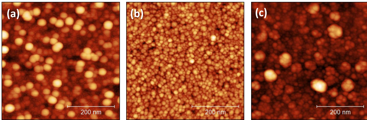
FIG. 1. Atomic force microscopy topographs of epitaxial InN films grown using plasma conditions which generate (a) low atomic N and low ion fluxes, (b) high atomic N and medium ion fluxes, (c) high atomic N and high ion fluxes.
