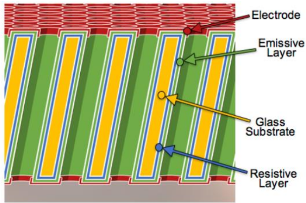
Schematic ALD-GCA-MCP structure (left) and its application as chevron pair in a photodetector (right).
