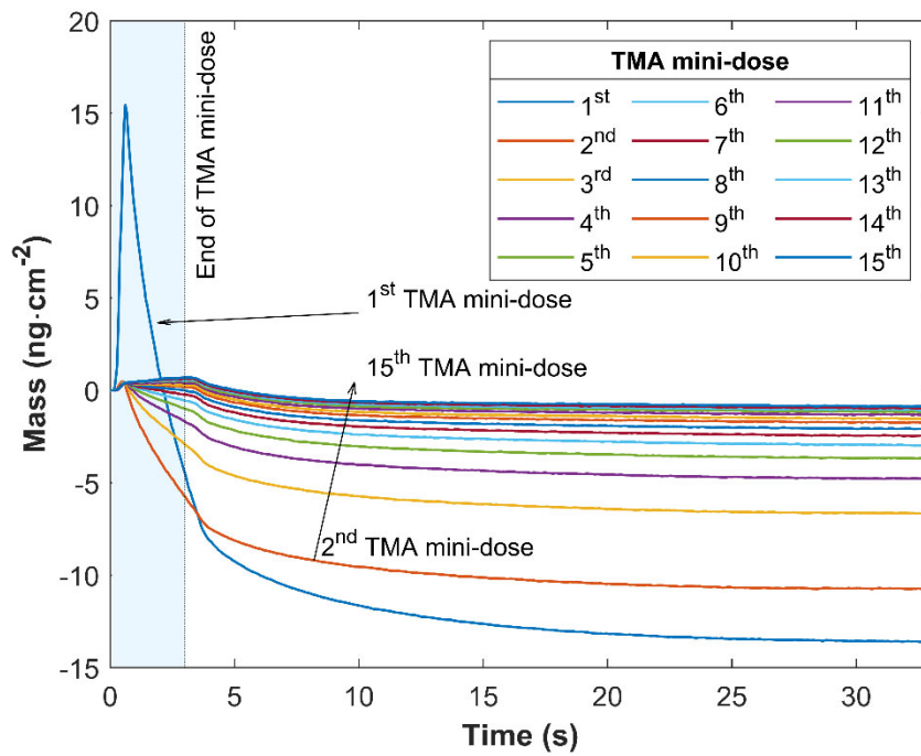
Figure 1 – QCM Response to successive mini-doses of TMA on HF-exposed Al 2 O 3 .
