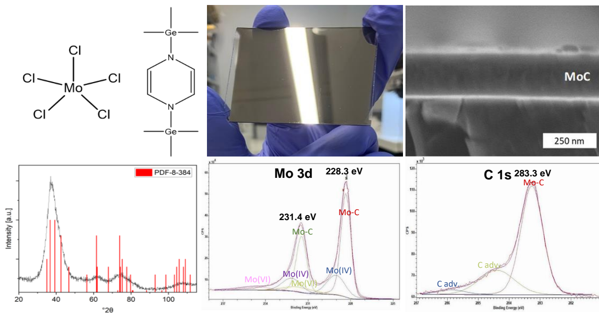
Figure 1: Top left: Structures of the precursors. Top middle: MoC film on soda lime glass. Top right: Cross-section SEM image of a 150 nm thick MoC film on Si substrate. Bottom left: XRD diffractogram from MoC film. Bottom middle: Mo 3d XPS spectrum of MoC film. Bottom right: C 1s XPS spectrum of MoC film.
