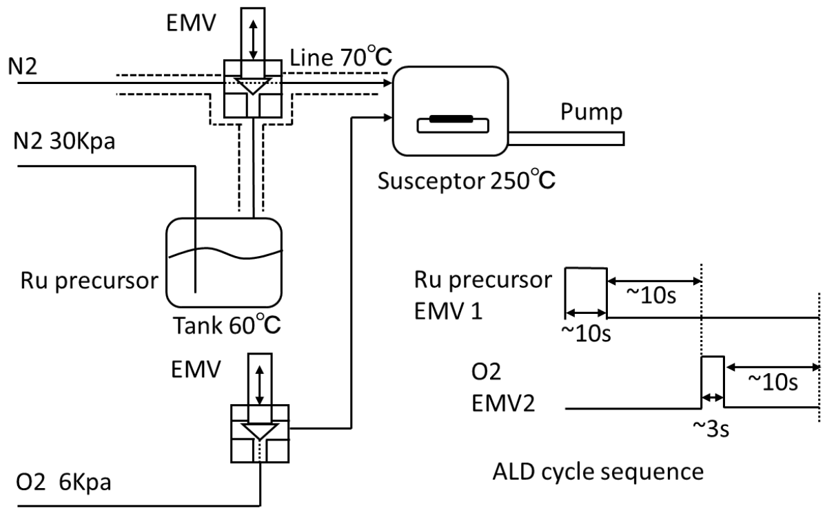
Fig.1 Tool configuration and setting
