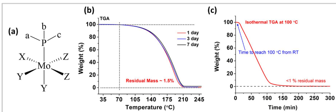
Figure 1: Mo (0) precursor (a) and its thermal stability (b), and isothermal behavior at 100 °C (c)
