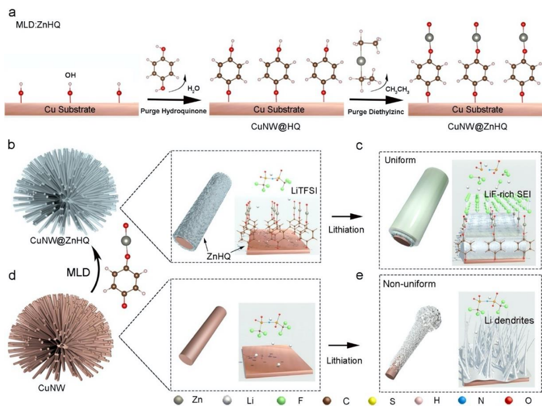
Figure 1 Schematic illustration of a) the chemical reactions in zincone MLD; b) SEI formation on CuNW@ZnHQ and c) Uniform Li deposition process under ZnHQ-induced Li-F rich SEI; d) SEI formation on CuNW and e) Non-uniform Li deposition process on CuNW.
