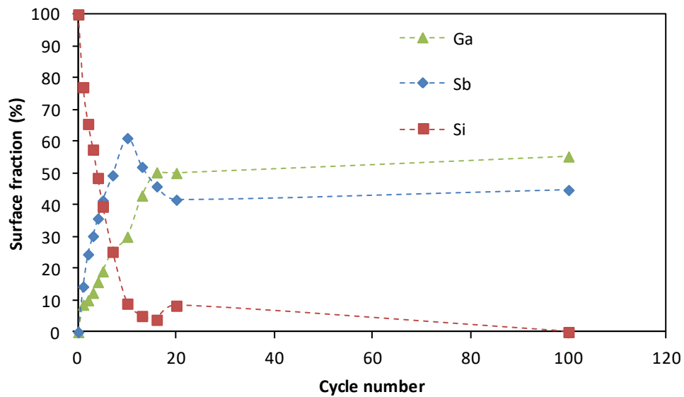
Figure 1: Surface fraction of Ga, Sb, Si and O as a function of cycle number
