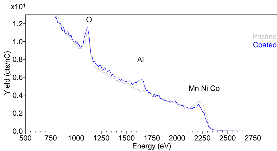
Figure 2a: 3 keV 4 He + LEIS spectra of pristine and AlO x coated NMC532 cathode material
