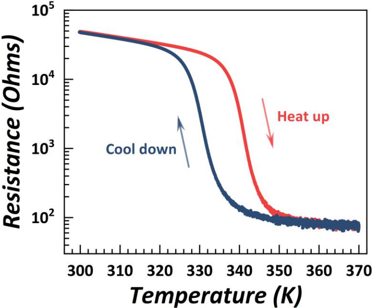
Supplemental figure. Temperature-dependent electrical measurement of the insulator-to-metal transition for the VO 2 thin film deposited by ALD.
