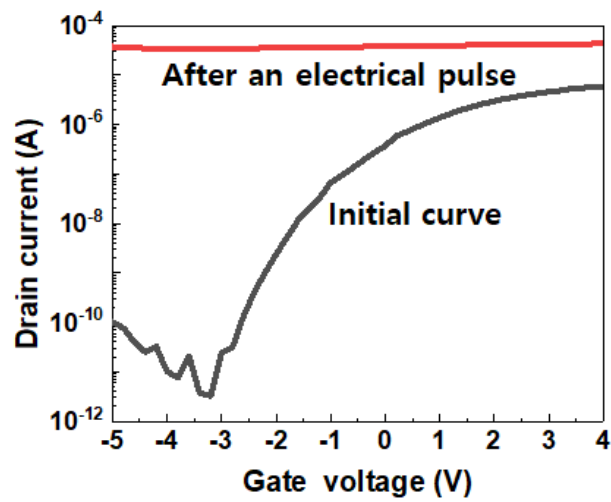
Fig. 2. Transfer curves of synaptic devices showing an initial curve and that after an electrical pulse
