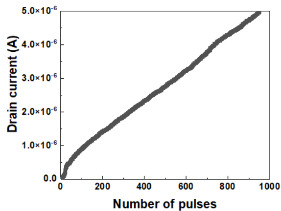
Fig. 3. The learning curves with applying repeated pulses with a short-term plasticity condition and 1024 states were obtained with good linearity.
