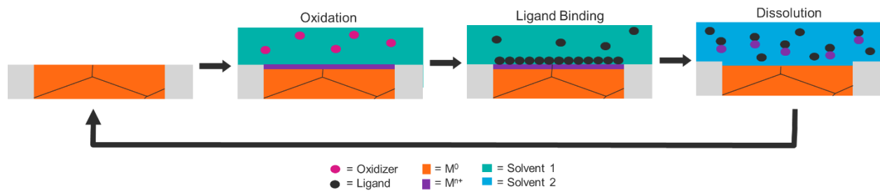
Figure 1. A diagram of wet ALE showing oxidation and ligand binding to form a surface complex, followed by selective dissolution of that complex in a different solvent.
