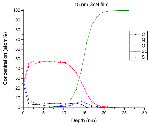
Figure 1: XPS Depth profile of PEALD ScN film.
