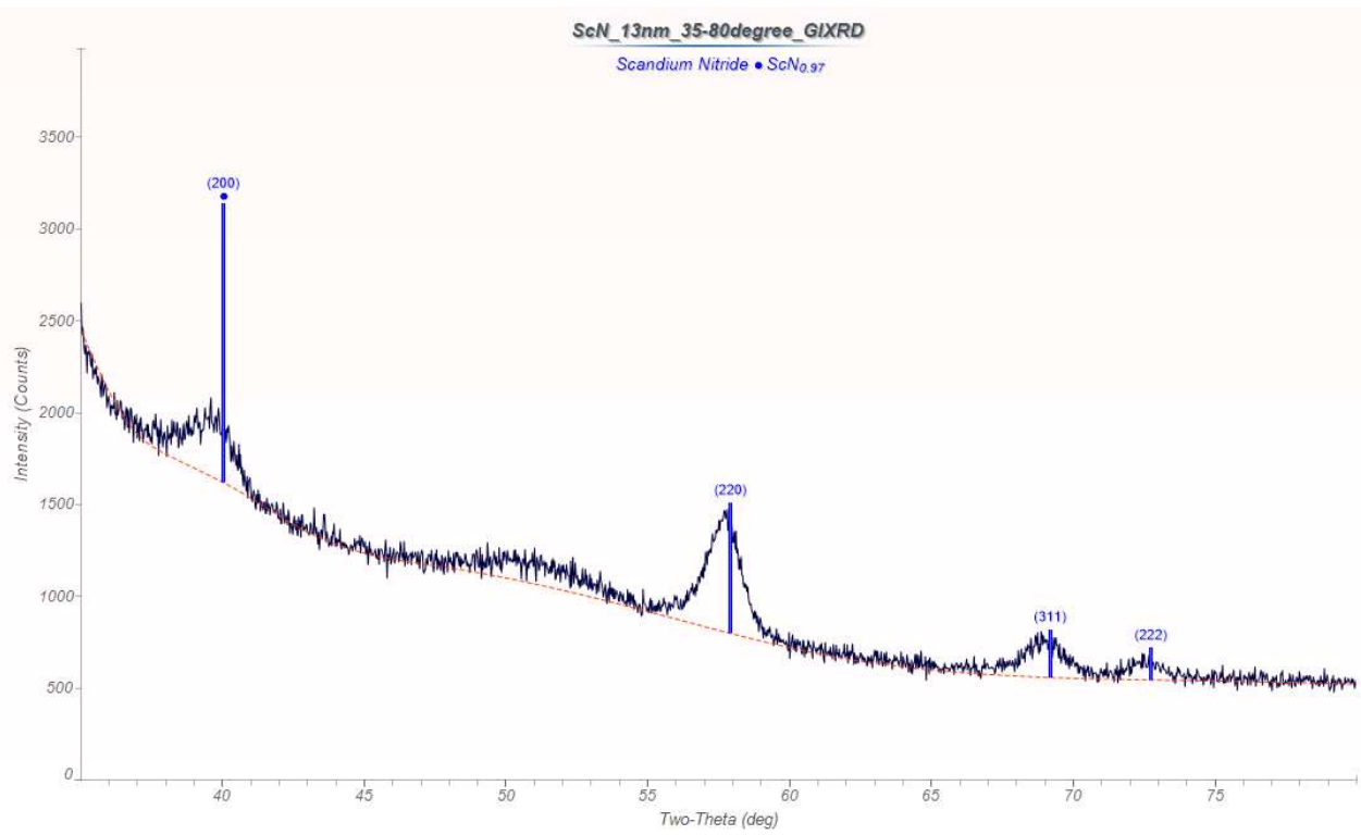
Figure 2: GIXRD of PEALD ScN film grown at 250°C with reference peak locations of cubic ScN.
