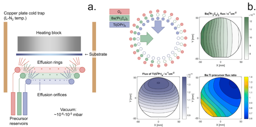
Figure 1. HV-CVD setup schematic and precursor flux simulation in a combinatorial mode.
