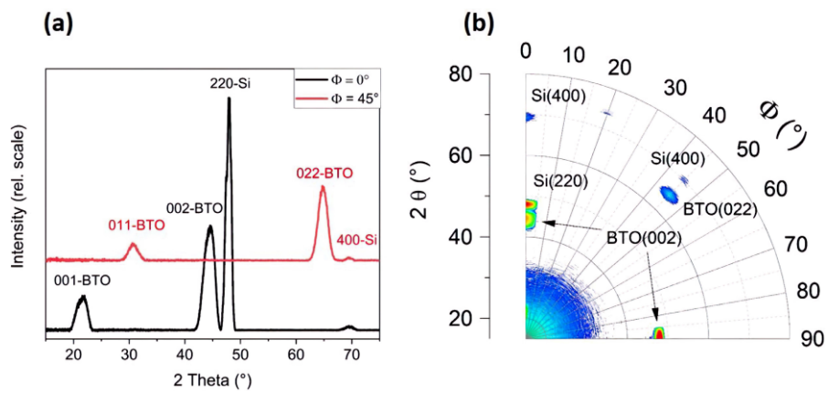
Figure 2. XRD texture analysis of BaTiO 3 on SrTiO 3 -buffered Si, reproduced from Borzi et al, Materialia , 2020.
