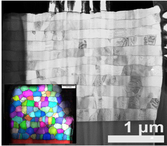
Figure 1. SEM cross-section image and TKD result of a deposited 2.5 \mu\text{m} thick Al-Al 2 O 3 multilayer thin film system displaying the brick-and-mortar microstructure.
