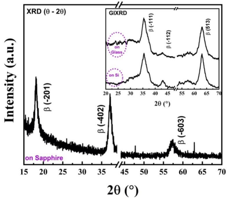
Figure 1. XRD spectra of 500-cycle grown \text{Ga}_2\text{O}_3 films using 50 W deposition and 250 W in-situ Ar-annealing plasma powers at 240 ^\circ\text{C} on sapphire substrate. Inset shows the GIXRD spectra of 500-cycle grown \text{Ga}_2\text{O}_3 films under the same conditions while on Si and glass templates.
