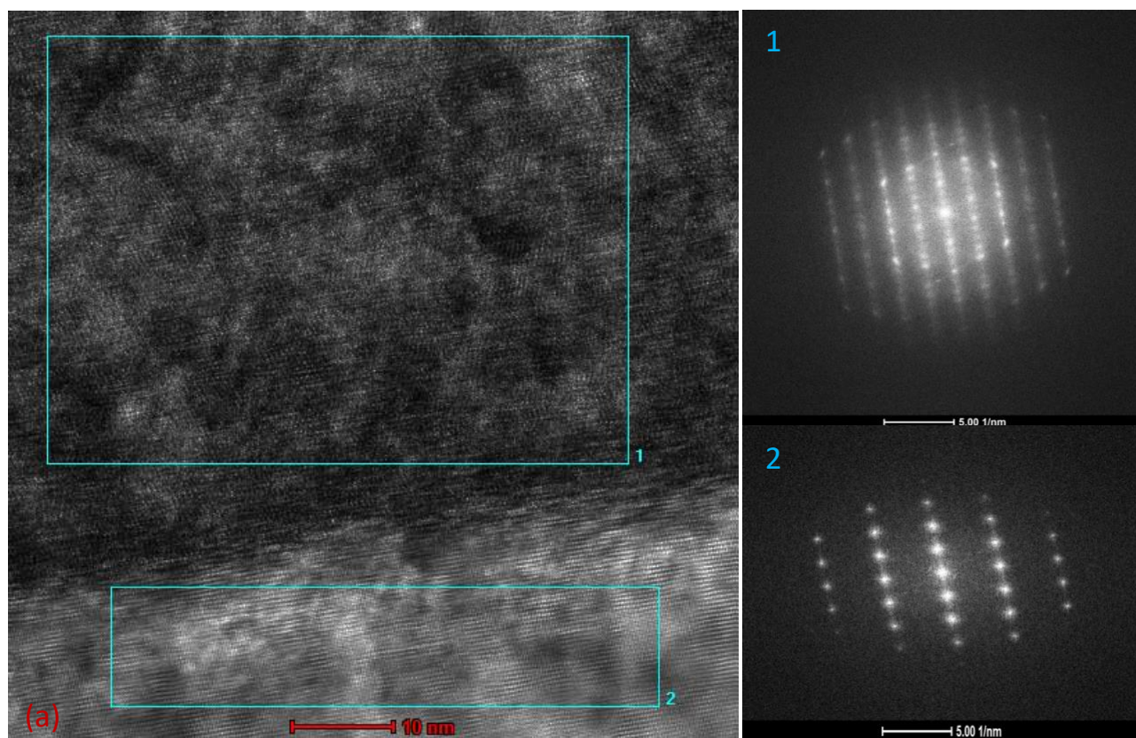
Figure 2. (a) HR-TEM micrograph of 500-cycle \text{Ga}_2\text{O}_3 sample grown at 240 ^\circ\text{C} substrate temperature on sapphire with 50 W \text{Ar}/\text{O}_2 plasma and 250 W in situ Ar-plasma annealing. Fast Fourier Transform (FFT) over the selected regions in (a), displaying dot-like patterns of the epitaxial structure (1) over the \text{Ga}_2\text{O}_3 layer and (2) over the sapphire substrate.
