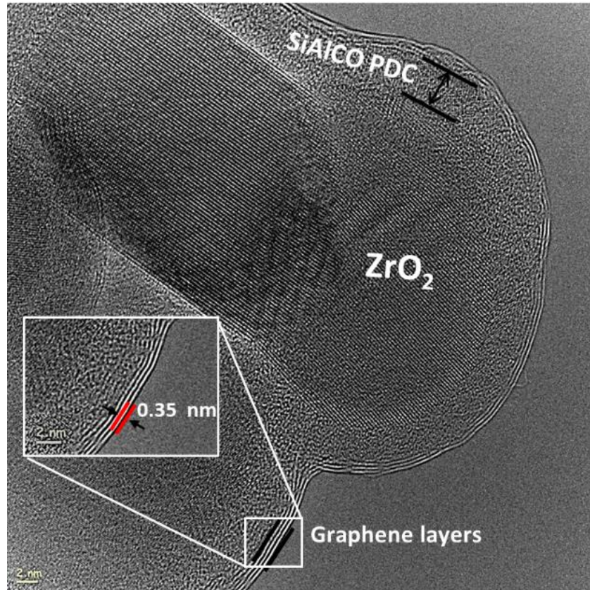
Figure 1. The HRTEM imaging of ZrO_2 nanoparticles coated with a 5 nm thick SiAlCO PDC film after vacuum annealing at 900^\circ\text{C} .
