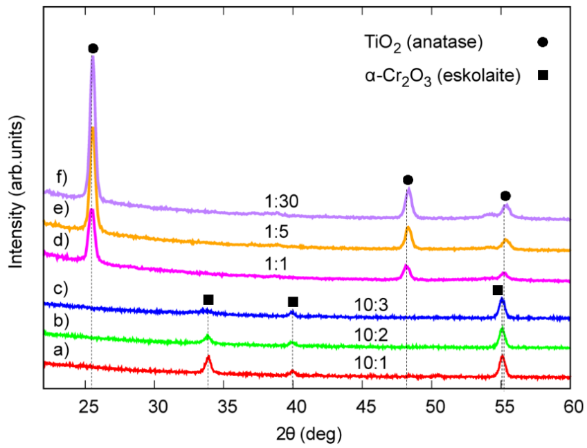
Fig. 1. Selected GIXRD patterns of Cr-Ti-O deposited thin films with different cycle ratio of [\text{CrO}_2\text{Cl}_2\text{-CH}_3\text{OH}] : [\text{TiCl}_4\text{-H}_2\text{O}] (a, b, c) and [\text{Cr}(\text{thd})_3\text{-O}_3] : [\text{TiCl}_4\text{-O}_3] (d, e, f).
